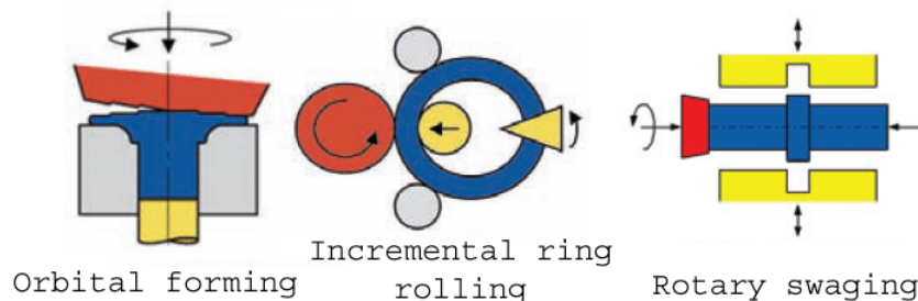
Fig.5. Some examples of incremental bulk forming
