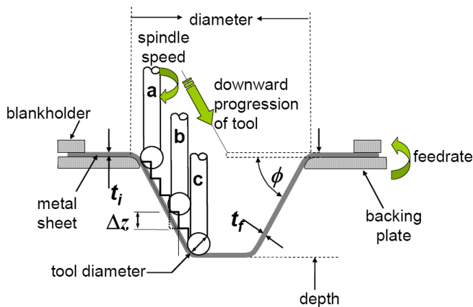
Fig.1. The principle of Single Point Incremental Forming [3]
