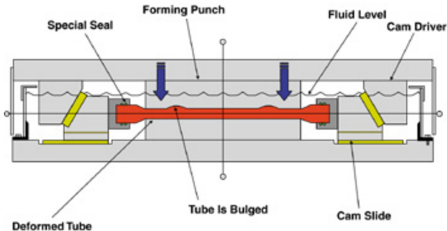
Fig.4. The principle of liquid impact forming [4]
