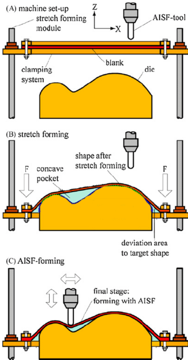
Fig.3. The principle of combined process [8]
