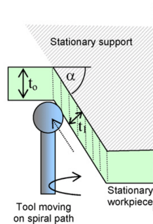
Fig.2. The principle of Two Point Incremental Forming [5]
