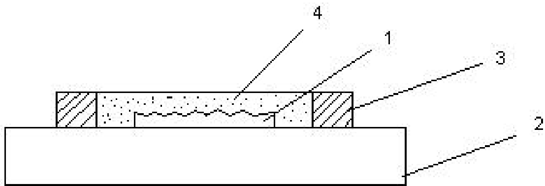
Figure 4. Obtaining of the silicone mould: 1-experimental primary model; 2-platform of the pressing machine; 3-polyurethanes frame; 4-silicone rubber mould
