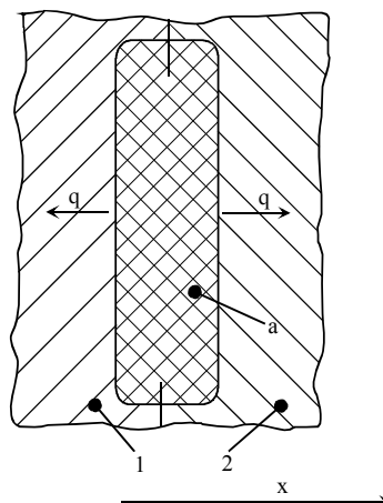
Fig.1. The thermal transfer in case of the injection pieces in mould: 1,2-forming plates; a- injected pieces; q-thermal high tide unitary on x direction. [7]
