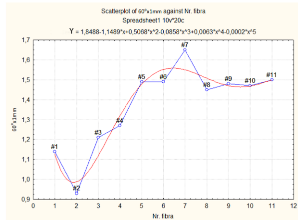
Fig.8 Variation of network size of material extruded with die 15°x7mm
