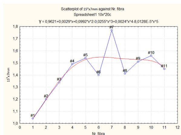
Fig.6 Variation of network size of material extruded with die 15°x7mm
