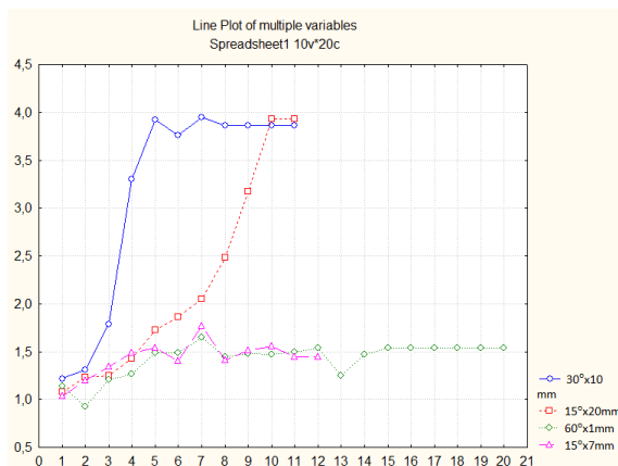
Fig.9 Comparative diagrams on the variation of the grid size
