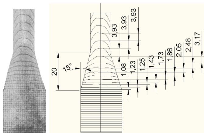
Fig.2 Die grid network 15°x20mm
