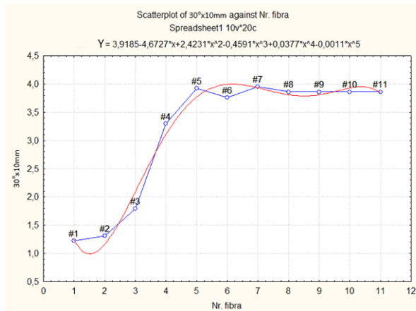
Fig.7 Variation of network size of material extruded with die 30°x10mm
