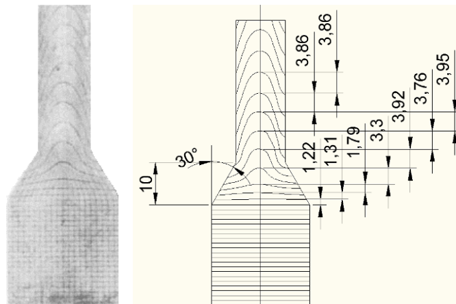
Fig.1 Die grid network 30°x10mm
