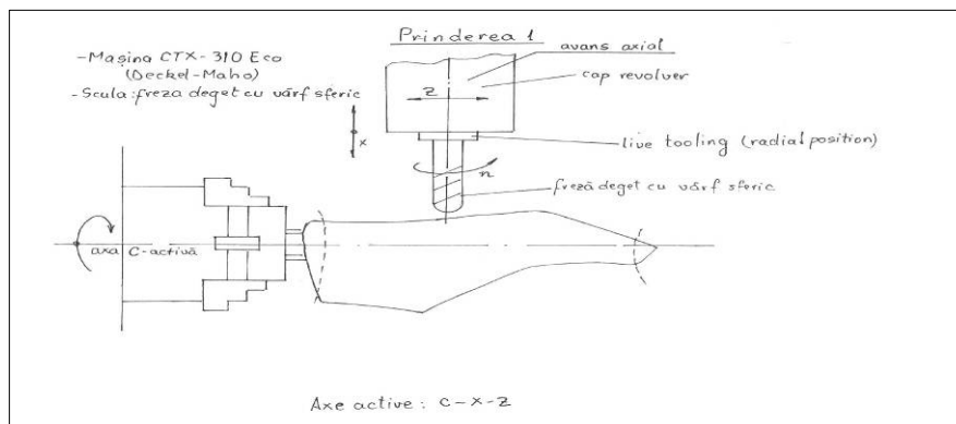
Figure 4 - Diagram representing milling machine on horizontal fixation last with finger-type cutter
