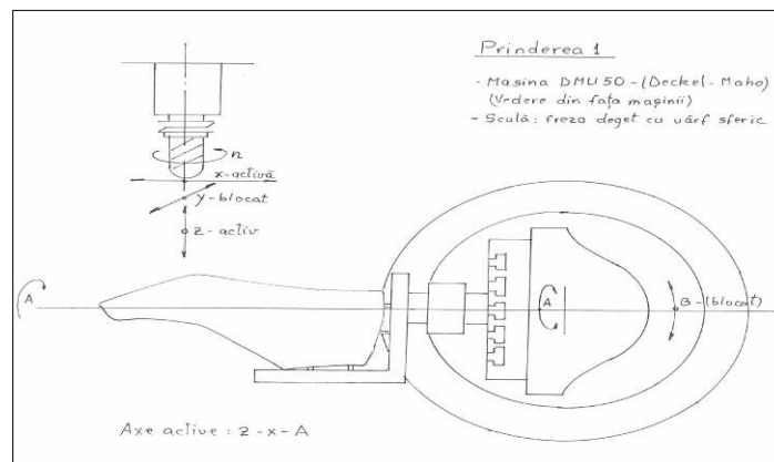
Figure 8 - Diagram representing milling machine DMU-50 on horizontal fixation last with finger-type cutter
