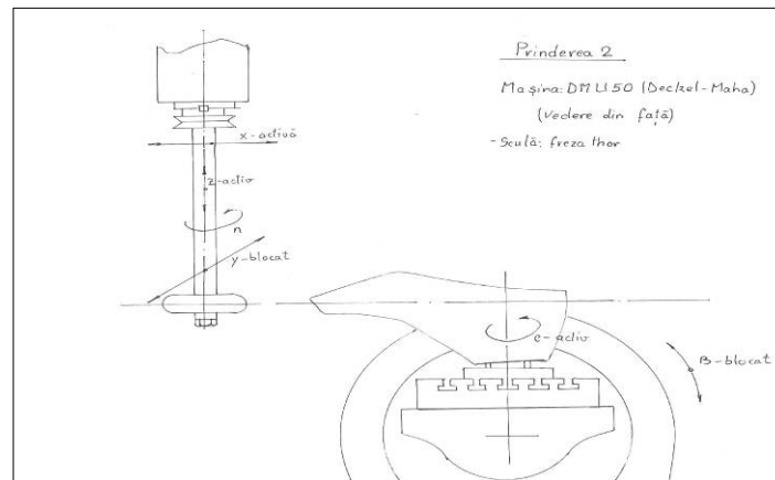
Figure 11 - Diagram representing milling machine DMU-50 with Live-Tooling device in horizontal fixation of the last
