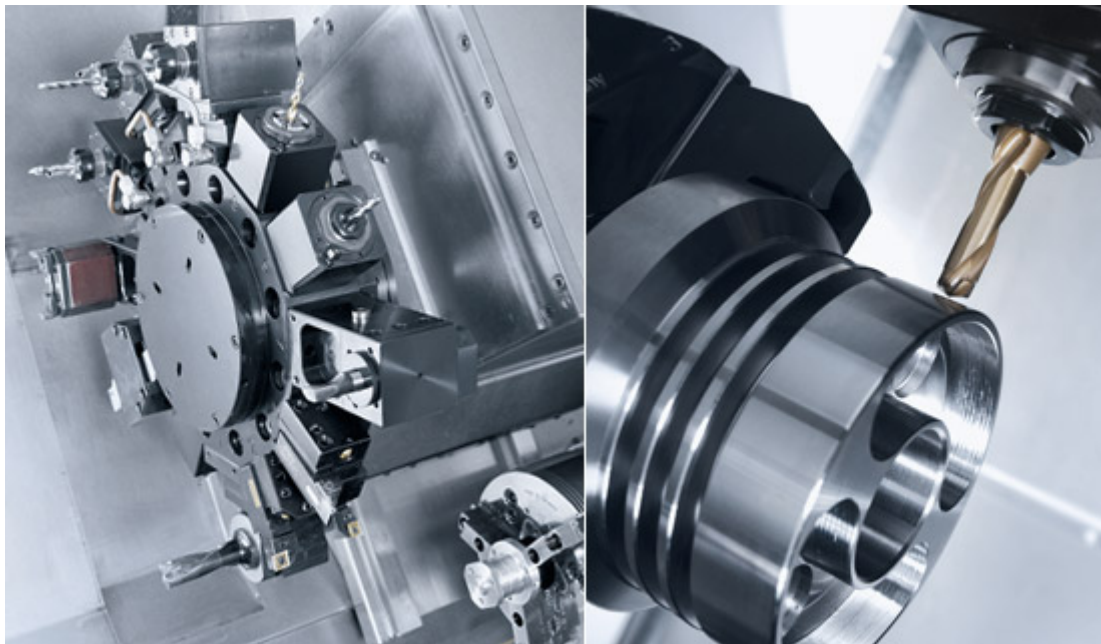
Figure 1- Live Tooling Milling head with different cutters and workpiece clamping jaw lathe
