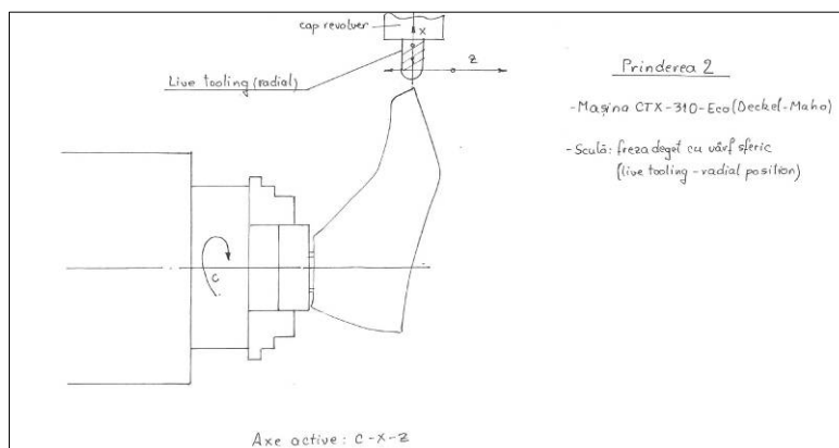
Figure 5 - Diagram representing milling machine on vertical fixation last with finger-type cutter
