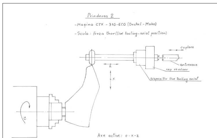
Figure 7 - Diagram representing milling machine with Live-Tooling device in vertical fixation of the last
