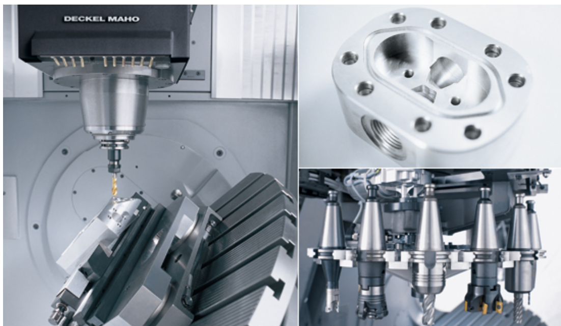
Figure 3 - Tilting rotary table and rotating the tool magazine
