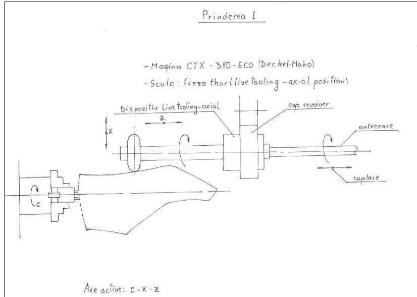
Figure 6 - Diagram representing milling machine with Live-Tooling device in horizontal fixation of the last
