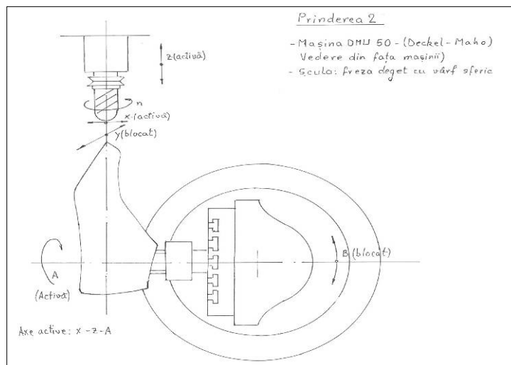
Figure 9 - Diagram representing milling machine DMU-50 on vertical fixation last with finger-type cutter
