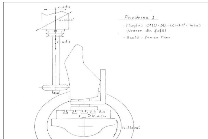
Figure 10 - Diagram representing milling machine DMU-50 with Live-Tooling device in vertical fixation of the last
