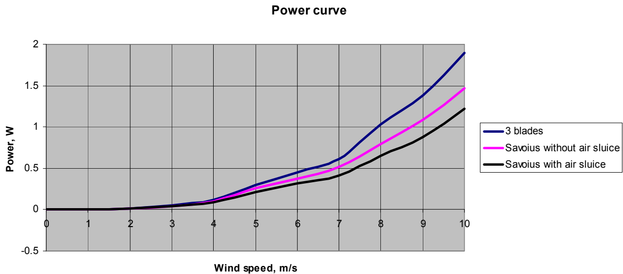
Figure 16: The power curve
