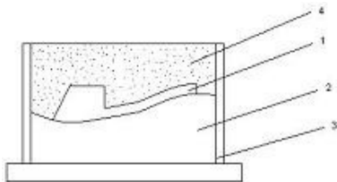
Figure 2. Cast obtaining 1-primary model of the sole; 2-base; 3-drain box; 4- cast
