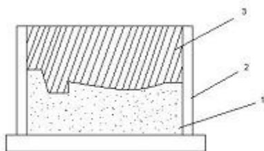
Figure 4. Obtaining of the non-metallic electrode: 1-cast; 2-drain box; 3-non-metallic electrode
