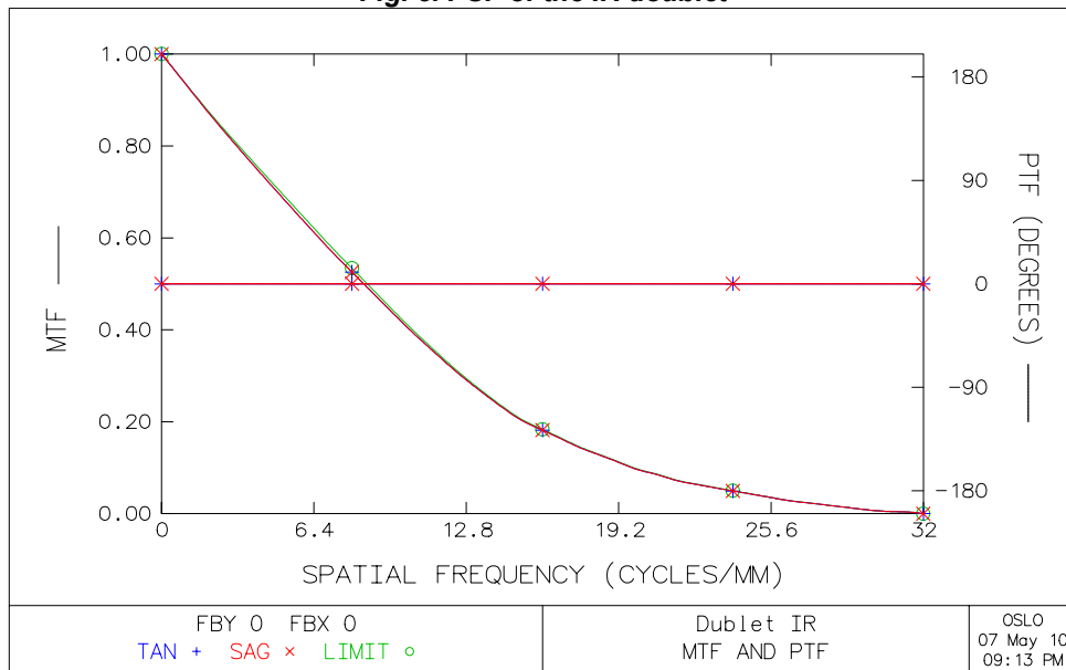
Fig. 6. MTF and PTF of the IR doublet
