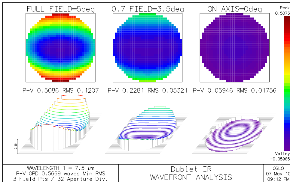
Fig. 3. Results of wavefront analysis of the IR doublet
