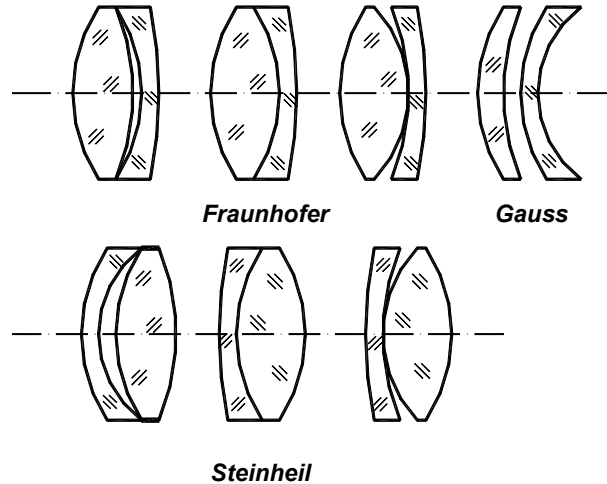
Fig. 1 Geometrical shapes of the doublet
