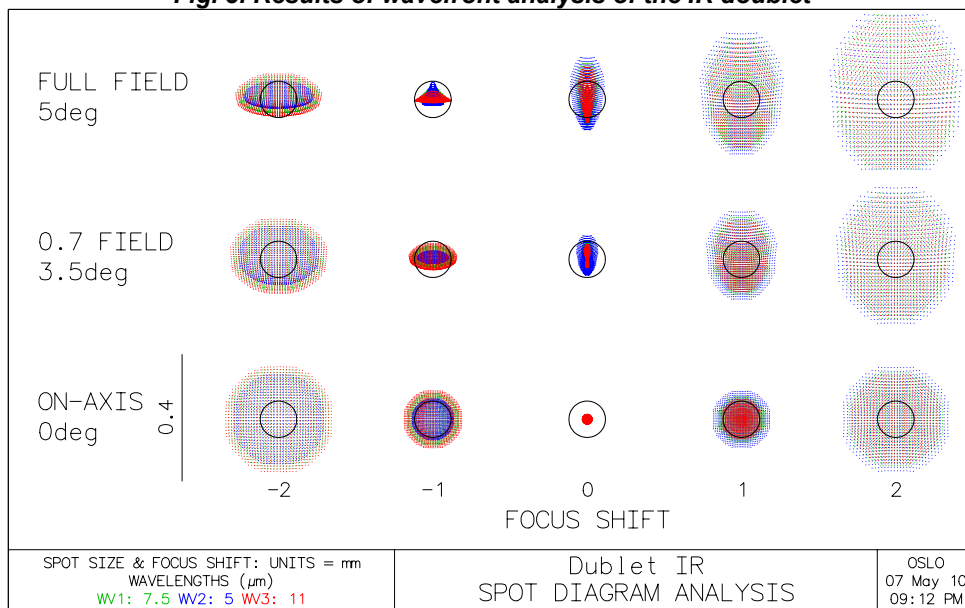
Fig. 4. Spot diagram for five focus abscissas and three field angles
