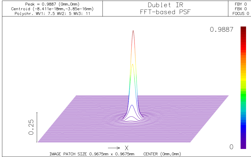
Fig. 5. PSF of the IR doublet
