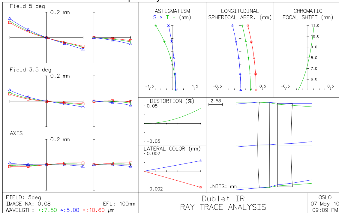
Fig. 2. Optical scheme, geometrical and chromatic aberrations of the IR doublet
