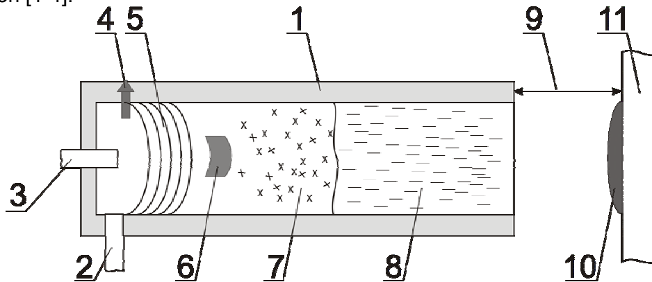
Fig.1. The scheme of detonation-gas coating application
