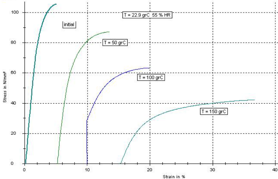
Fig.2 The curve of the properties of PA 66 material
