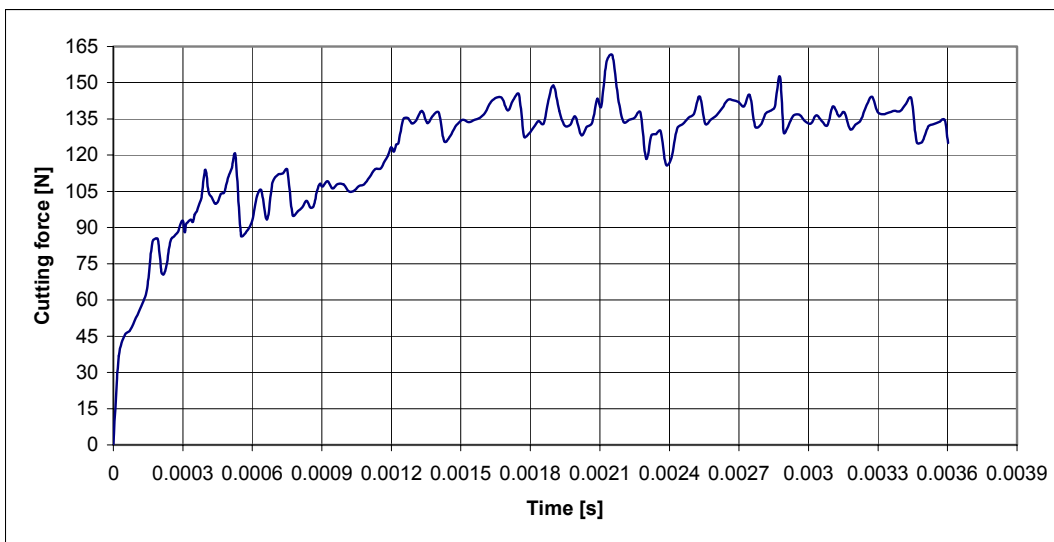
Fig. 4 The cutting force F_z - a_p = 2 mm, f = 0,4 mm/rev, v = 235 m/min
