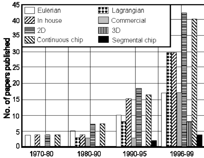
Fig.1 Research trends in finite element modelling [26]
