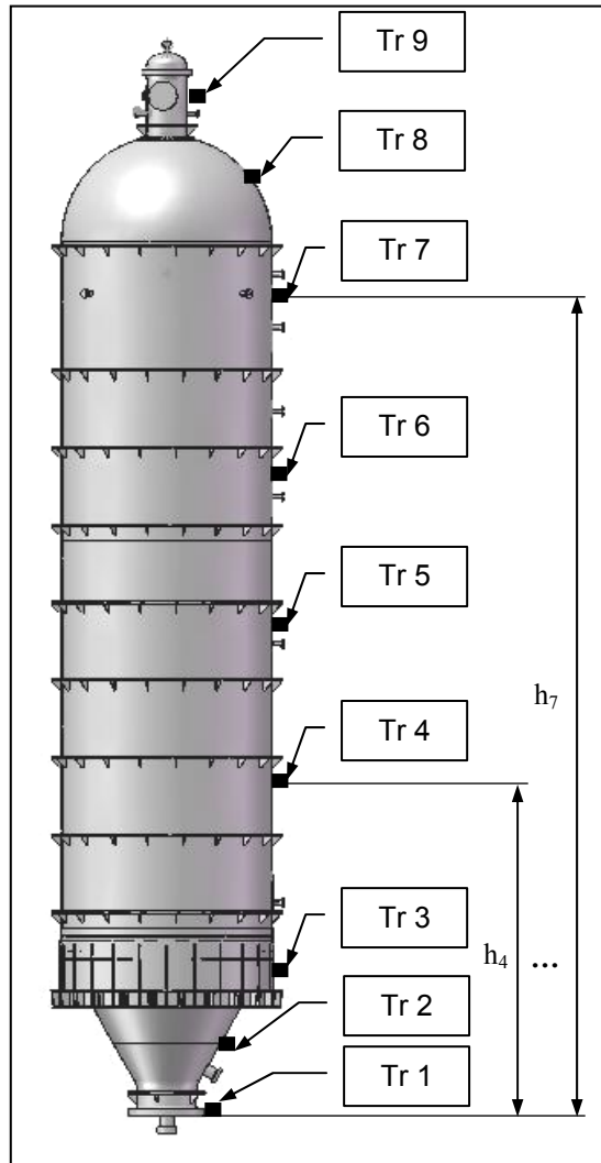
Figure 2: The vertical mounting dimensions for the sensors' placement
